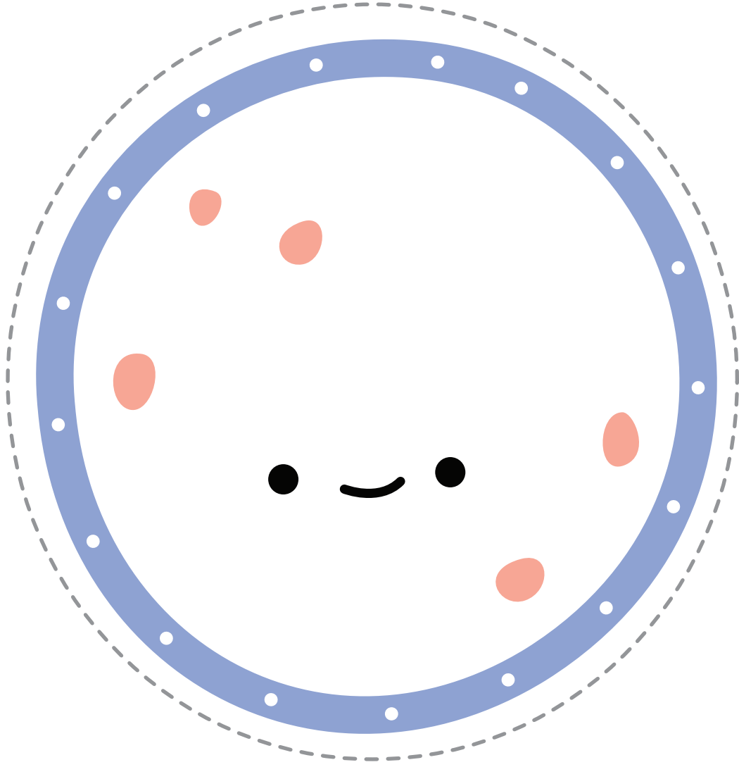
mercury
